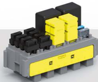
Accepts 20 MiniVal fuses or 20 circuit breakers or 20 diodes or 6 Micro 280 relays or mixed
