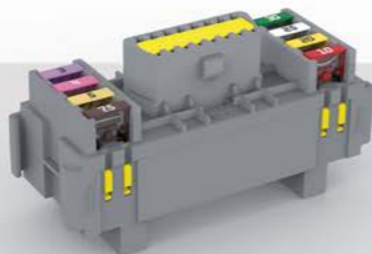
Accepts 8 MiniVal fuses and 1 OBD connector
